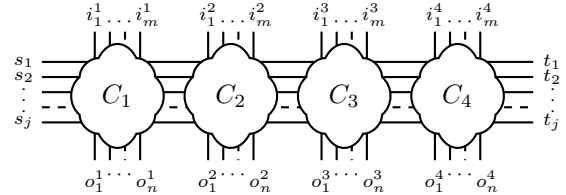
Fig. 1: Unfolded circuit encoding four execution cycles
