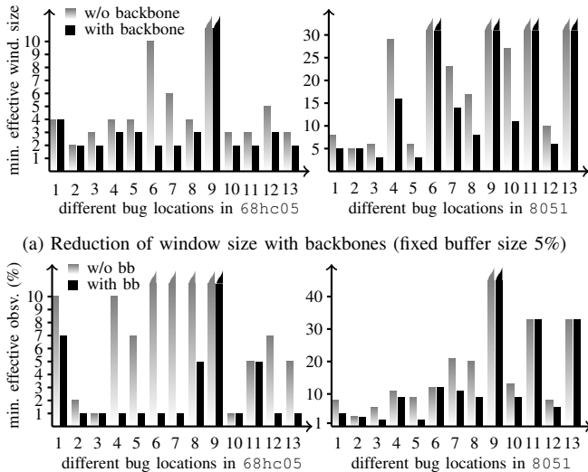
(b) Reduction of trace buffer size with backbones (using a fixed window size of 3 for the 68hc05 and 5 for the 8051 design)
